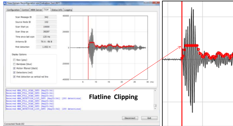
Fig. 9: Example of clipped or flatlined detections.
