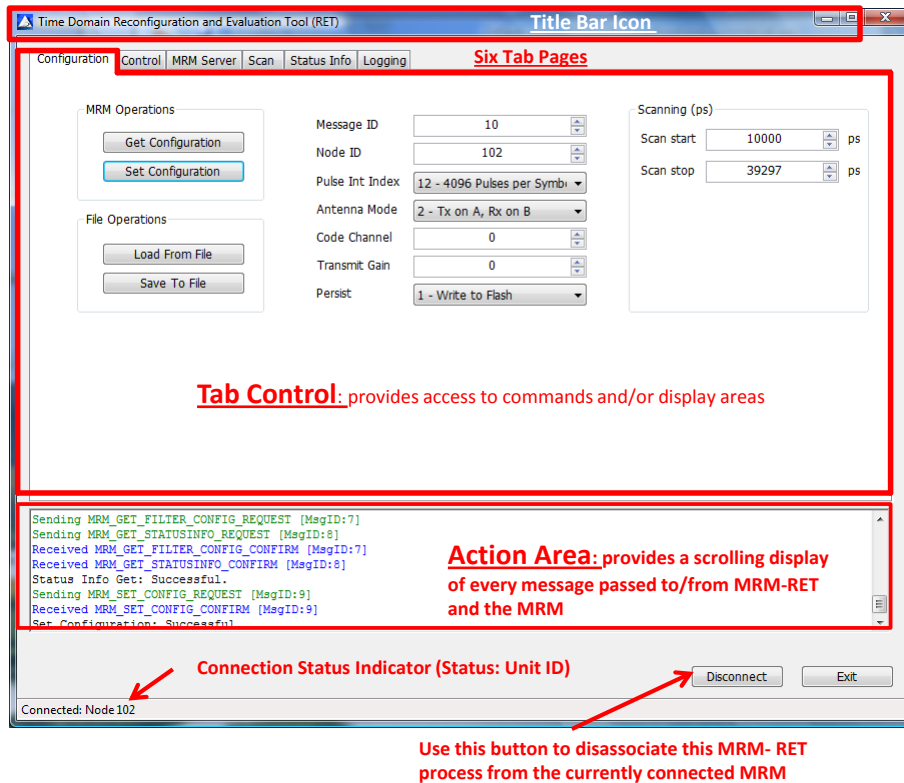
Fig. 3: Configuration screen with indication of the main areas
