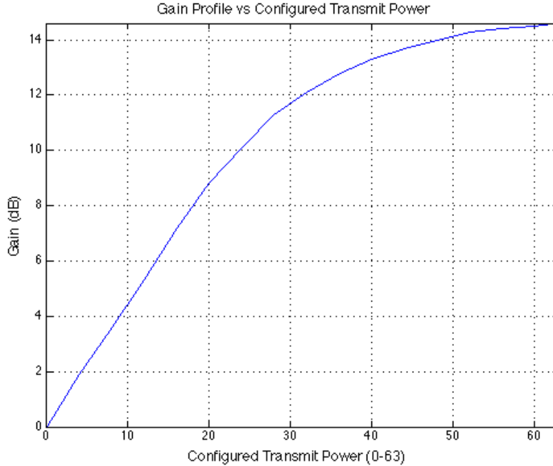
Fig 5: Relationship of Transmit Gain value to transmit power
