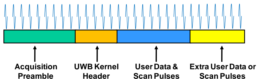
Fig. 2: Allocation of pulses in a notional packet (not to scale)
