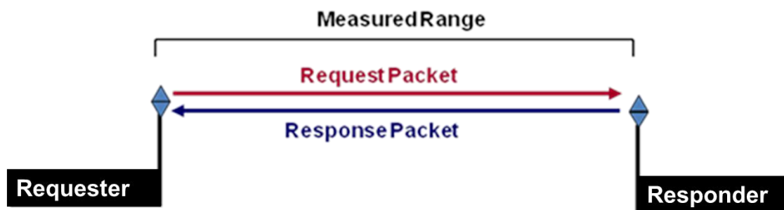
Fig. 1: Packet transmissions required by TW-TOF range measurement
